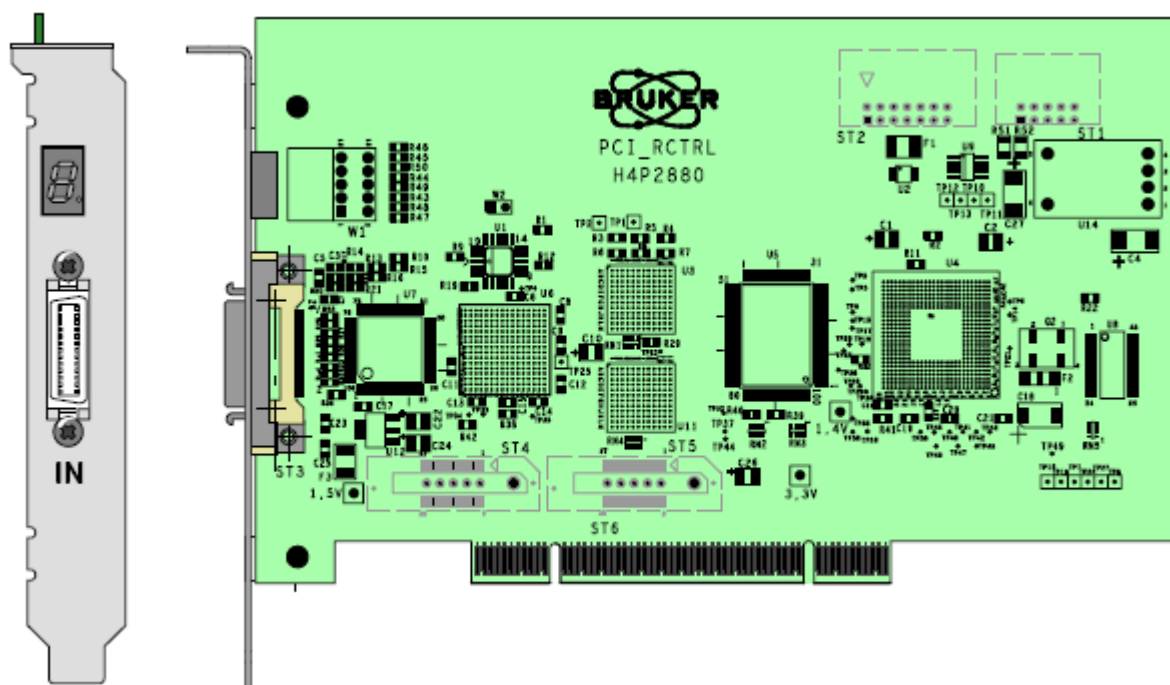
Figure 1.1. Rx-Controller Front and Top View
