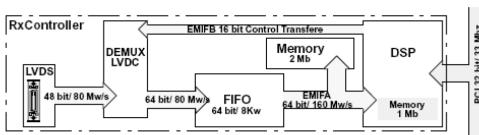
Figure 4.1. The Rx-Controller
