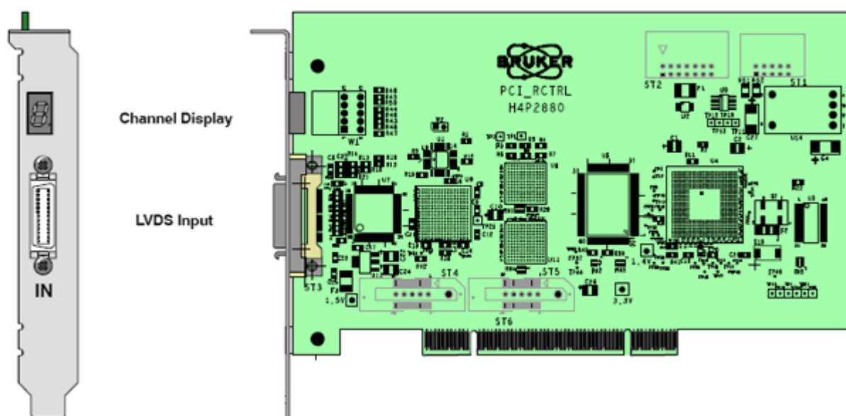
Figure 4.2. PCI Rx-Controller
